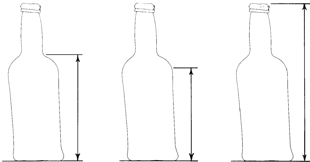
Figure 80. Body/shoulder height.
