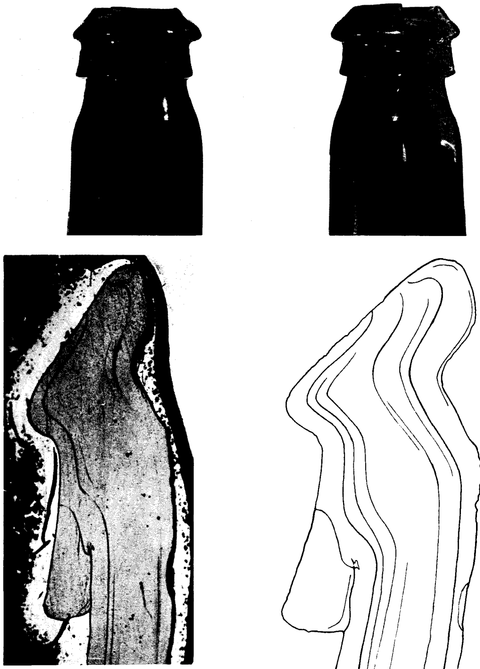
Figure 7. Tooling of crack-off surface has given this lip a down-tooled profile. Groove in the bore is less severe than in Fig. 8. (Thin section and photo by K. Allen; drawing by D. Kappler; photos by G. Lupien; RA-5166B, RA-5165B)
